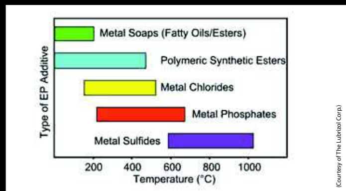
Figure 1. Activation Temperatures for Various EP Additives
